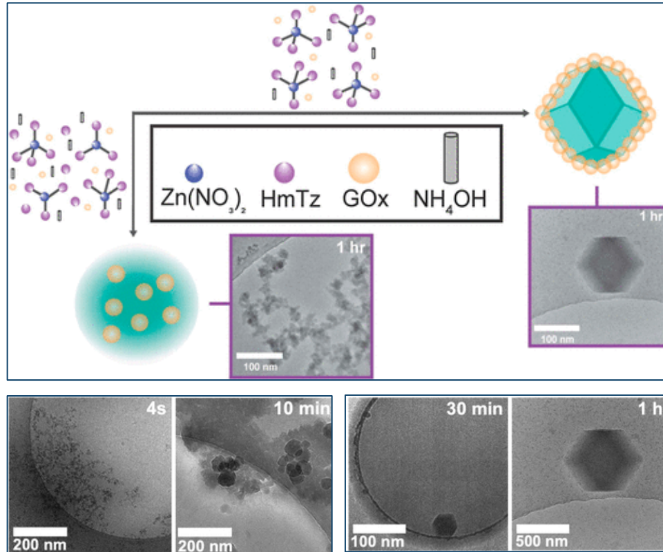
Figure: Nucleation and growth studies were conducted using time-resolved cryo-TEM to establish the crystallization mechanism for metal azolate framework-7 (MAF-7).
